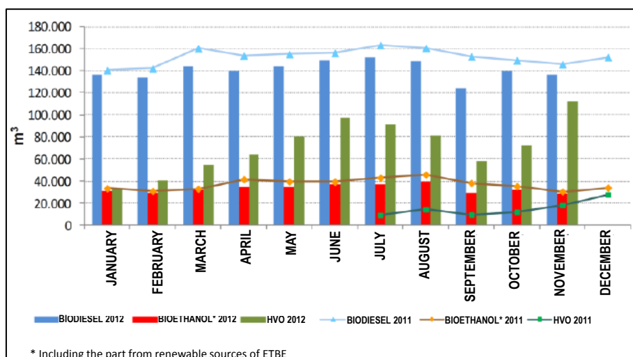
Fig. 3 Sales of Biofuels as of November 2012 (Source: CNE)
