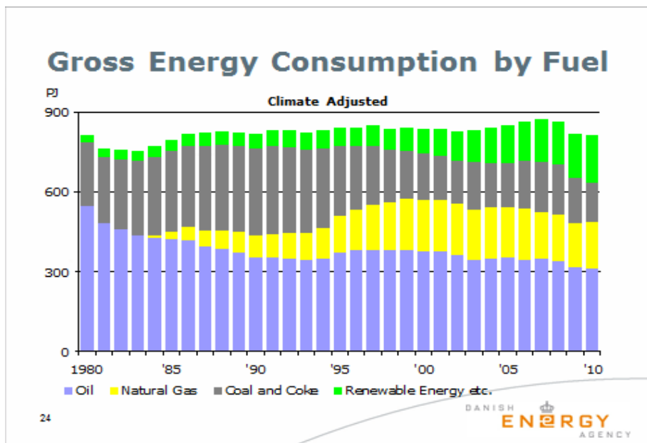
Fig. 1 Gross Energy Consumption by Fuel
