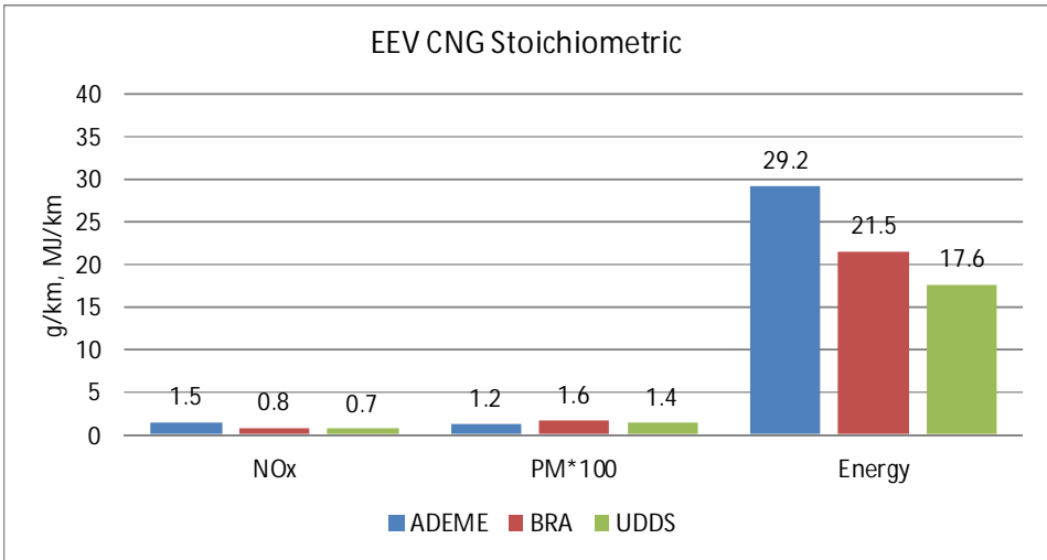
Figure 2.6. The effect of driving cycle on NO x , PM and fuel consumption. EEV CNG stoichiometric.
