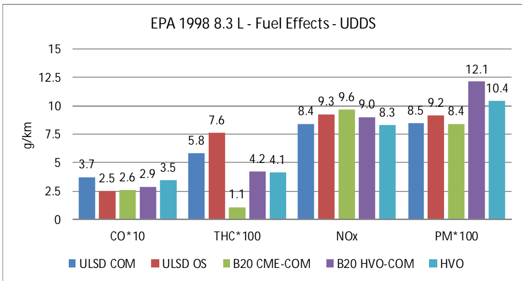
Figure 12.13. Fuel effects on regulated emissions. EPA 1998 8.3 L.
