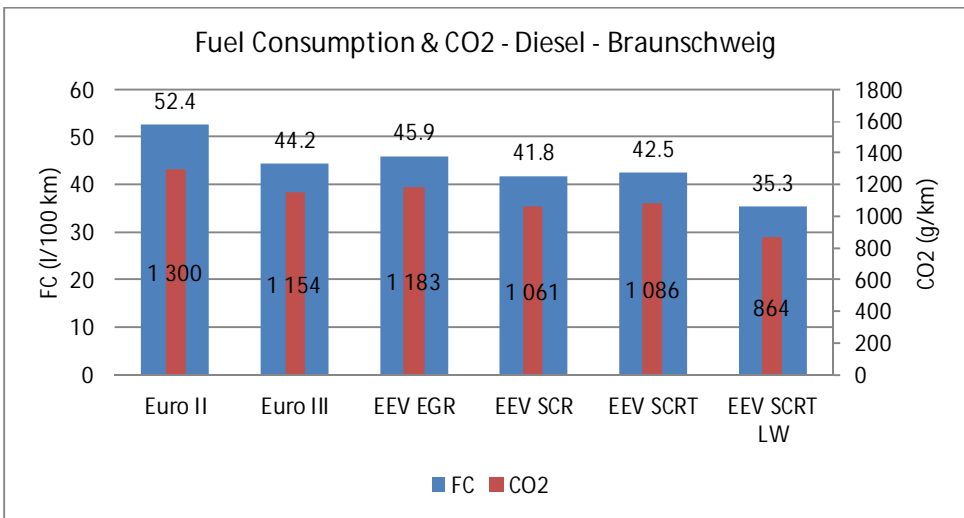
Figure 12.34. Fuel consumption (l/100 km) and CO 2 emissions for diesel vehicles with conventional powertrains. European vehicles, Braunschweig cycle.
