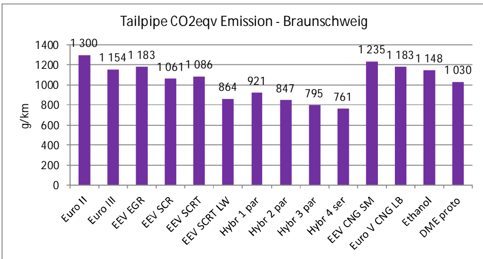
Figure 12.41. Tailpipe CO 2 eqv emissions of all tested European vehicles. Braunschweig cycle. CH 4 taken into account with a factor of 21 for CNG, ethanol and DME.
