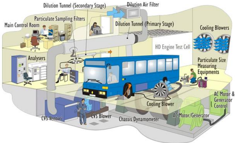
Figure 8.4. Schematic of VTT's heavy-duty test facility.
