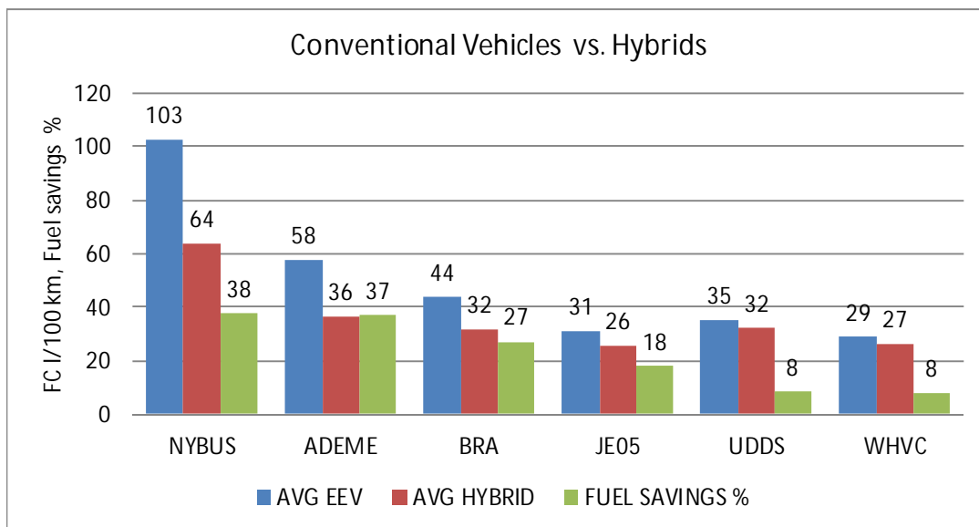
Figure 12.50. The effect of hybridization on fuel consumption.
