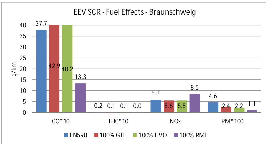
Figure 12.67. Fuel effects on CO, THC, NO x and PM emissions. EEV SCR diesel.
