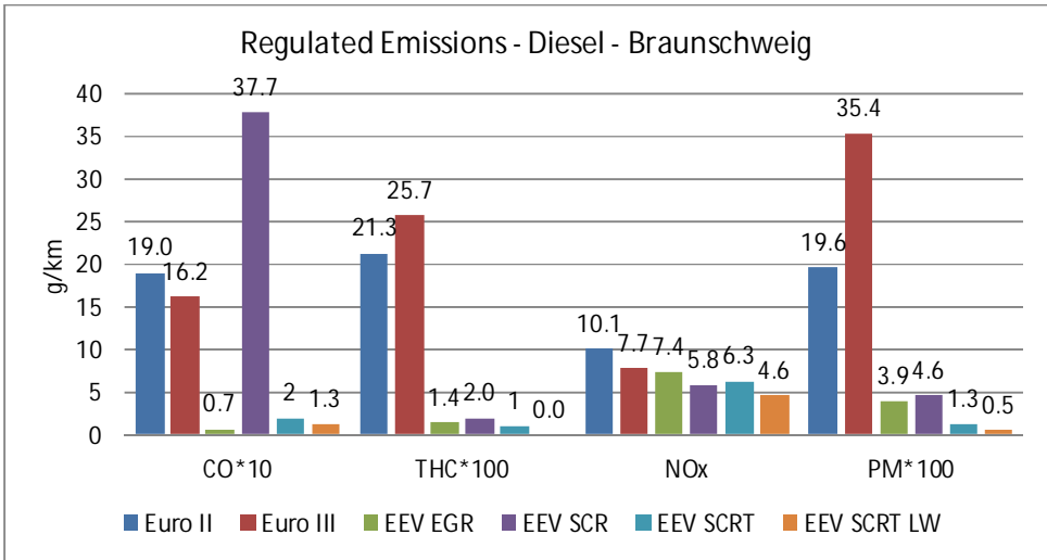
Figure 12.33. Regulated emissions for diesel vehicles with conventional powertrains. European vehicles, Braunschweig cycle. N.B.: The PM emission of the tested Euro III vehicle was rather high, average value of corresponding vehicles (same model) tested at VTT is some 0.20 g/km.
