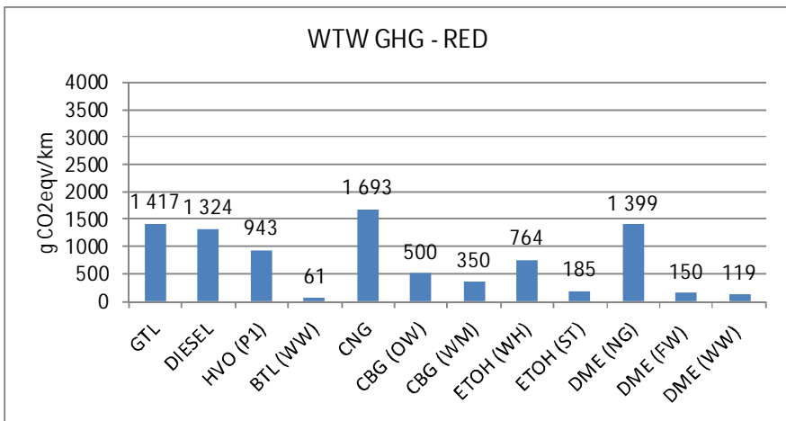
Figure 13.4. WTW GHG emissions for SCRT diesel and alternative fuel vehicles. RED methodology. Braunschweig cycle.
