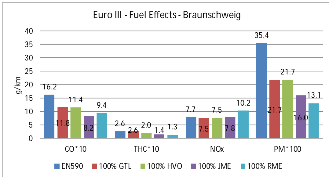
Figure 12.63. Fuel effects on CO, THC, NO x and PM emissions. Euro III diesel.
