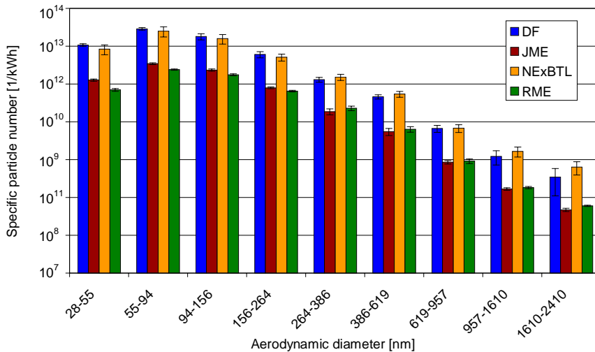
Figure 12.95. Specific particle number distribution in raw exhaust gas (ELPI, ESC test, OM 906).
