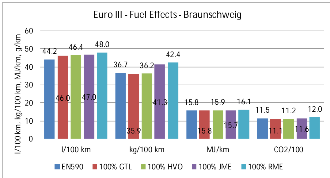
Figure 12.64. Fuel effects on volumetric and gravimetric fuel consumption, energy consumption and tailpipe CO 2 emissions. Euro III diesel.
