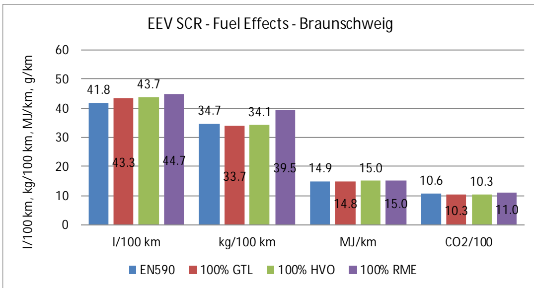
Figure 12.68. Fuel effects on volumetric and gravimetric fuel consumption, energy consumption and tailpipe CO 2 emissions. EEV SCR diesel.
