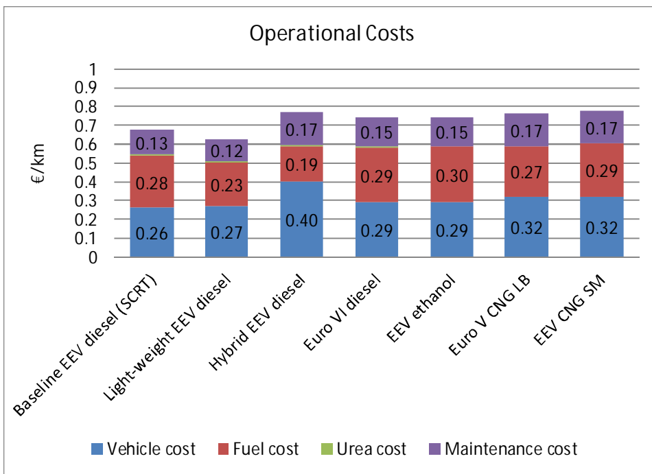
Figure 2.15. Operational costs (indicative) for various vehicle options. Baseline assumptions.
