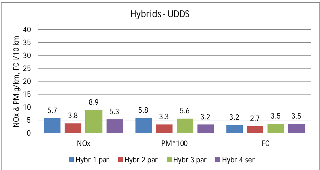
Figure 12.55. NO x , PM and fuel consumption for the hybrid buses. UDDS cycle.
