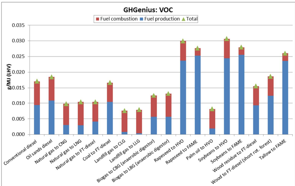
Figure 11.16. Lifecycle VOC Emissions from GHGenius.
