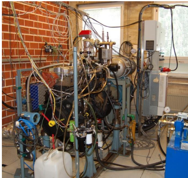
Figure 2. LEO research engine used in the ReFuel high-speed engine runs.
