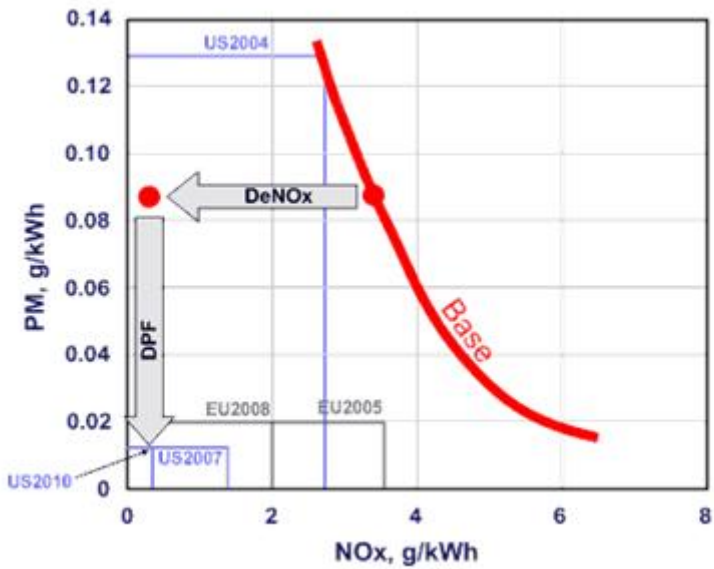
Figure 7.6. Emission control strategy for US 2010. De-NO x most probably a combination of EGR and SCR. (Majewski/DieselNet 2007)
