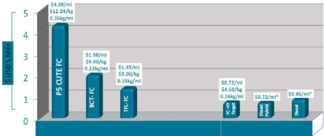
Fig. 5. Fuel costs for fuel cell and diesel/diesel-hybrid transit buses. To become competitive with conventional transit buses will require improvements in fuel cell efficiency and hybridization strategies, and a considerable reduction in the cost of H 2 .
