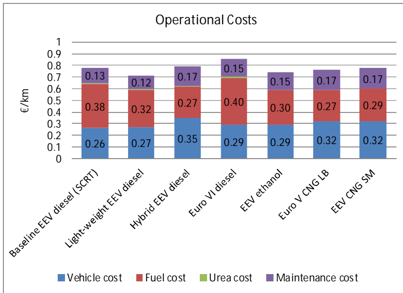
Figure 14.18. Operational costs (indicative) for various vehicle options. Diesel price 0.90 €/l, price of the hybrid vehicle 290,000 €
