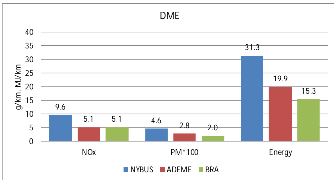
Figure 12.60. The effect of driving cycle on NO x , PM and fuel consumption. DME vehicle.
