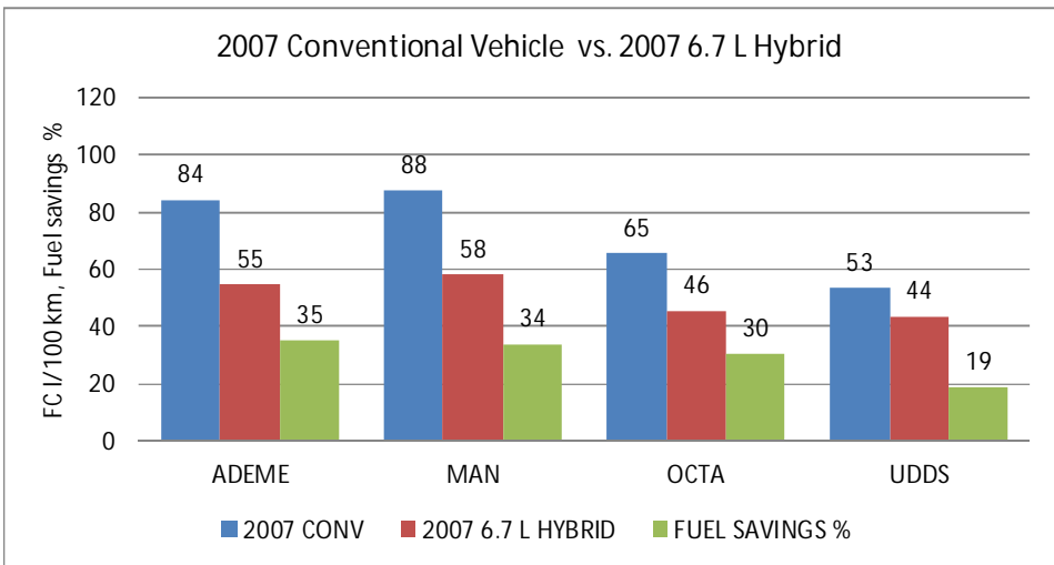
Figure 2.7. An example of driving cycle and hybridization on fuel consumption.
